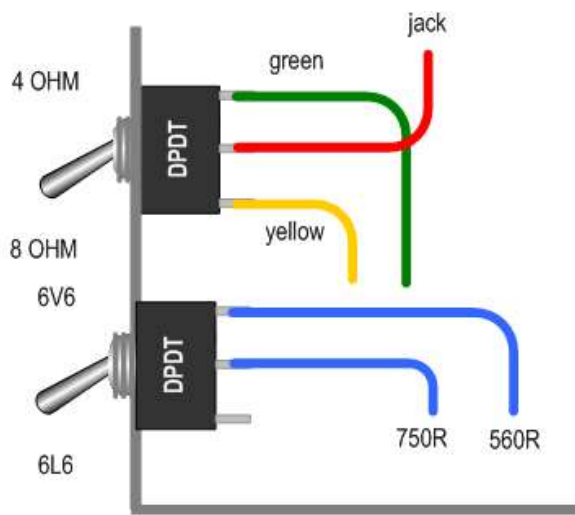
Side View of Switches
